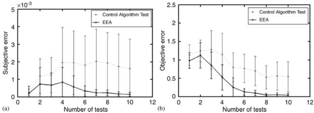
Figure 9. (a) Subjective error versus number of tests; and (b) objective error versus number of tests. Results are for EEA and control algorithm. Case for no noise and three sensors.
