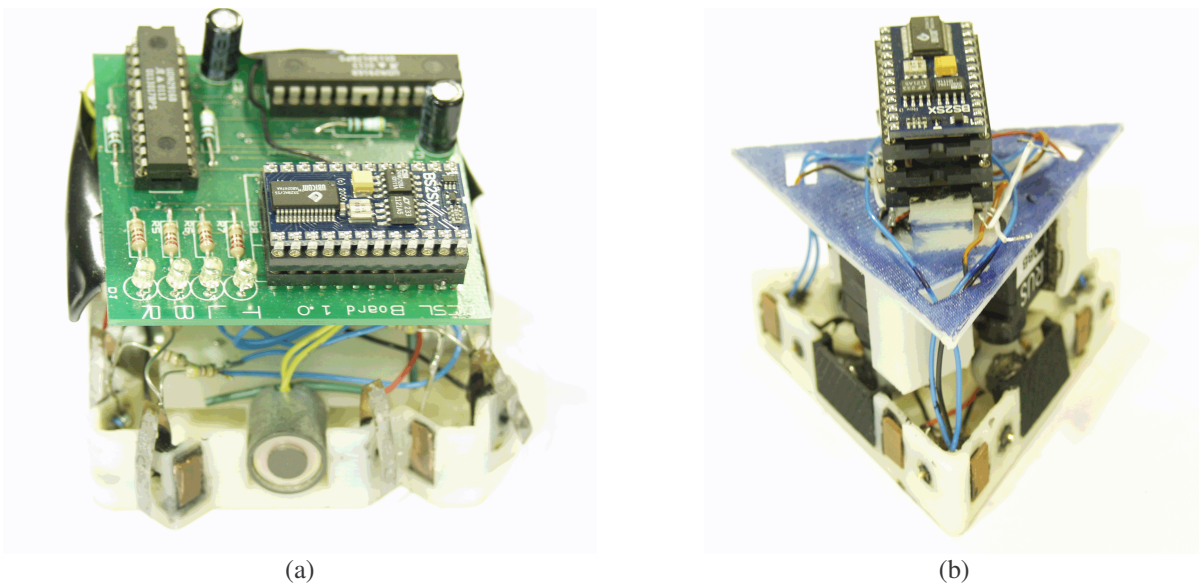
Figure 2. Two prototype units (a) square, using electromagnets (b) triangle, using swiveling permanent magnets
