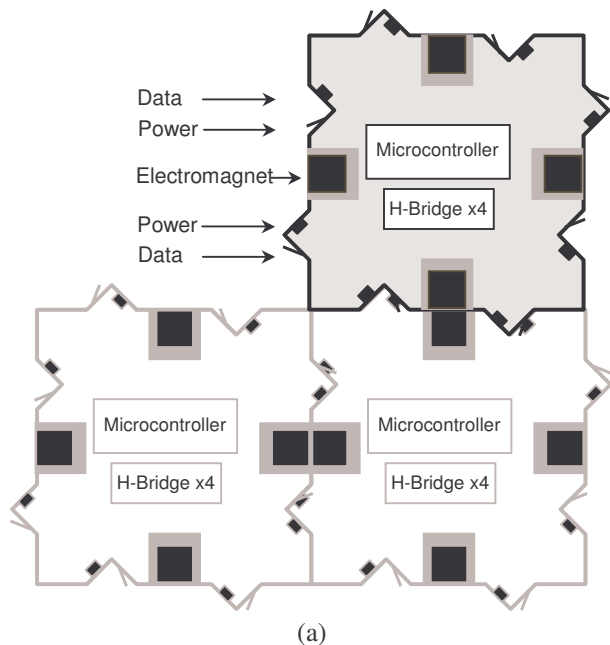
Figure 3. Design of a unit cell (a) Layout and I/O schematics, (b) base geometry
