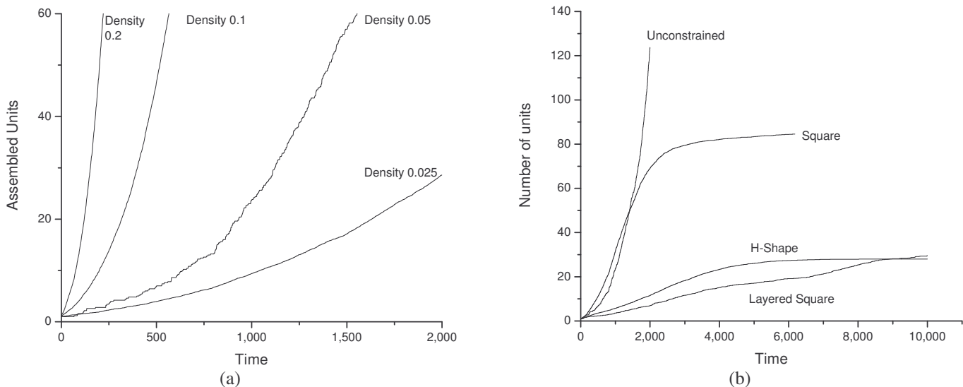
Figure 6. Self-configuration rates. (a) unconstrained geometries under four densities; (b) Comparing different control schemes for reconfiguration with density 0.05: Uncontrolled, 10x10 square, 10x10 square with growth rate control, and H-structure with diameter equivalent to a 10x10 square. Time units are arbitrary.
