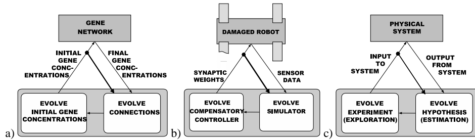
Fig. 2. Instantiations of the estimation-exploration algorithm. a: In order to reverse engineer a genetic network, the estimation phase evolves a connection matrix that describes the wiring of the network. Based on the best evolved connection matrix hypothesis, an input vector is evolved by the exploration phase that should return an information-rich output vector when applied to the hidden network. b: A neural network controller is evolved for an actual robot (exploration phase) that allows it to move. If it suffers damage, the estimation phase evolves a robot simulator that explains the damage. c: The general framework for applying the algorithm to a nonlinear system.
