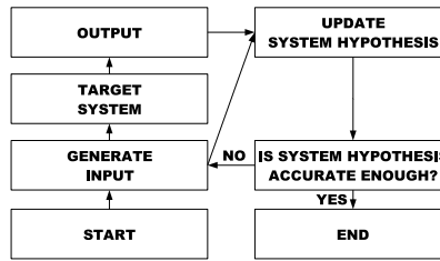
Fig. 1. Flow of a generalized reverse engineering algorithm.
