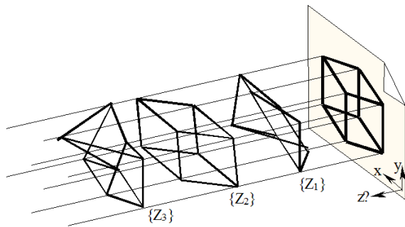
Figure 2: A sketch provides only two of the coordinates (x, y) of object vertices. A 3D reconstruction must recover the unknown depth coordinate z . In parallel projections, this degree of freedom is perpendicular to the sketch plane; there are an infinite number of candidate objects – the problem is indeterminate. Each candidate object is represented by a unique set of Z coordinates, e.g. sets \{Z_1\} , \{Z_2\} and \{Z_3\}
