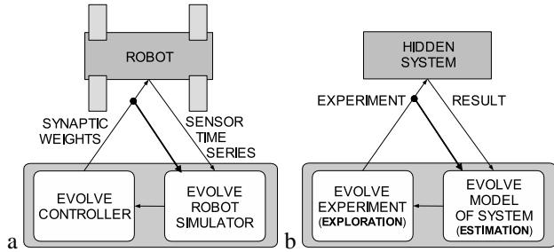
Figure 1: Schematic view of the proposed algorithm. a: The cyclical flow of the estimation-exploration algorithm, as applied to evolutionary robotics. The exploration phase evolves controllers in simulation and transfers them to a target robot; based on sensor time series and the evolved controller, the estimation phase improves the simulation. b: The general layout of the algorithm for inferring the structure of some hidden target system.
