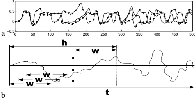
Figure 3: a: The three lines represent the time histories of one of the simulated robot’s angle sensors: each time history corresponds to three different simulated robots using the same controller. Only the first 500 time steps of the 1000 time step evaluation period are shown. The thick line indicates the angle sensor’s values when one of the robot’s motors is weakened by 10%; the line with circle markers when the same motor is weakened by 20%; and the line with triangle markers when one of the touch sensors is weakened by 50%. b: Outline of the rolling mean fitness metric.
